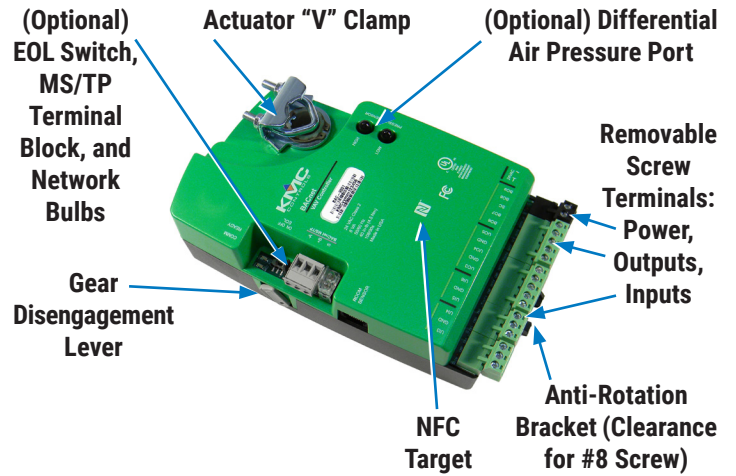
(BAC-9001AC with MS/TP shown)
