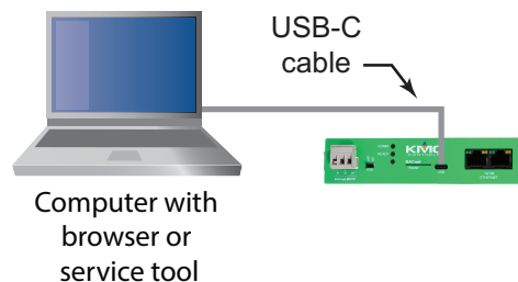
Illustration 1–6 Single-cable connection
