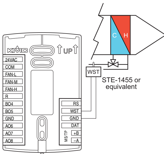
Illustration 2-6 Wiring for a water temperature sensor
