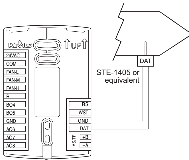
Illustration 2-4 Wiring for Discharge Air Temperature Sensor
