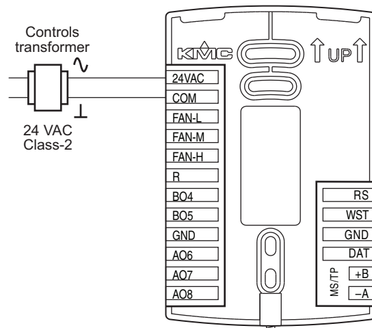
Illustration 2-13 Wiring for AppStat power
