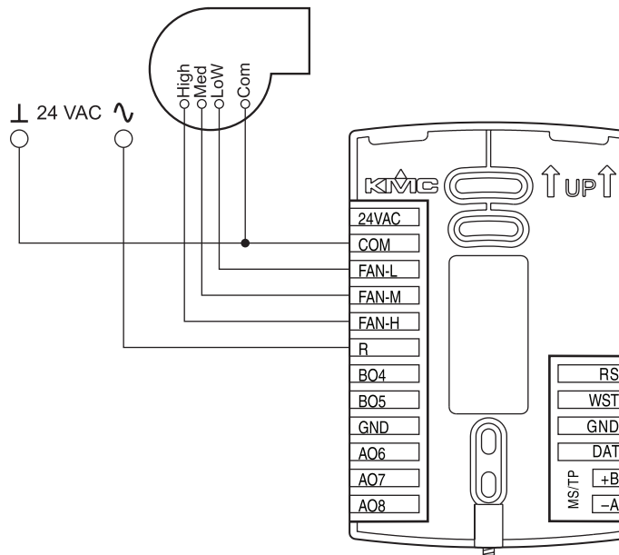
Illustration 2-8 Connections to a three-speed fan
