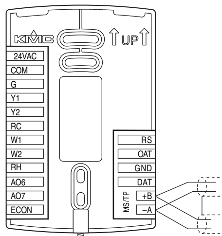
Illustration 7-1 BACnet MS/TP network wiring
