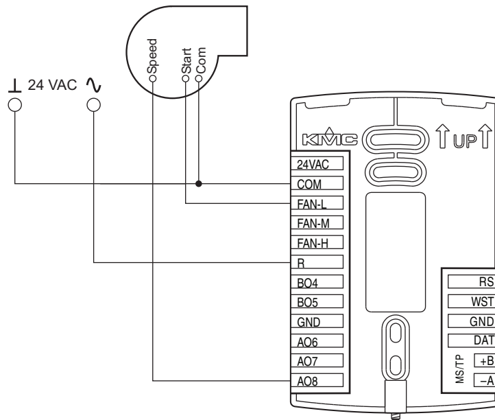
Illustration 2-9 Connections for a modulating fan
