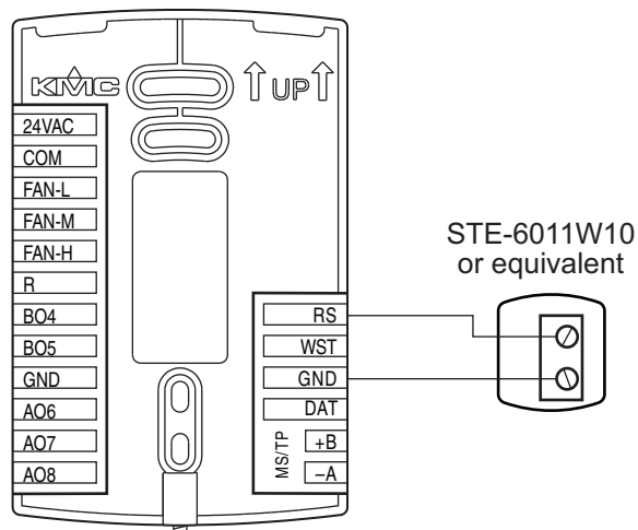
Illustration 2-3 Wiring for remote space temperature sensor
