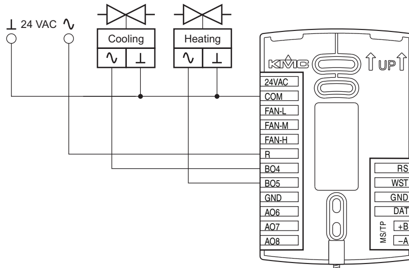
Illustration 2-10 Connections to on/off valves
