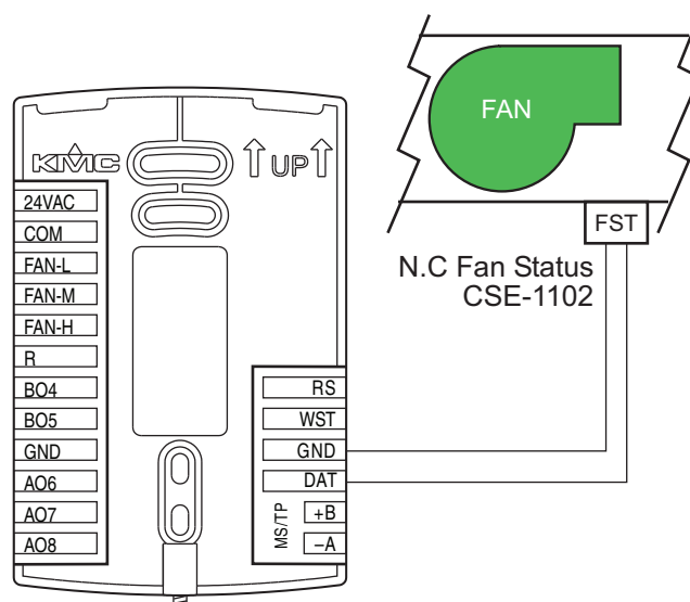
Illustration 2-5 Wiring for a fan status switch
