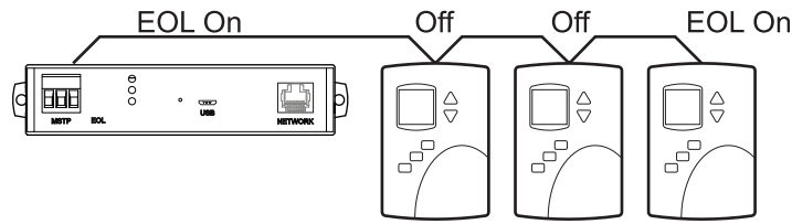
Illustration 7-2 Location for end-of-line termination
