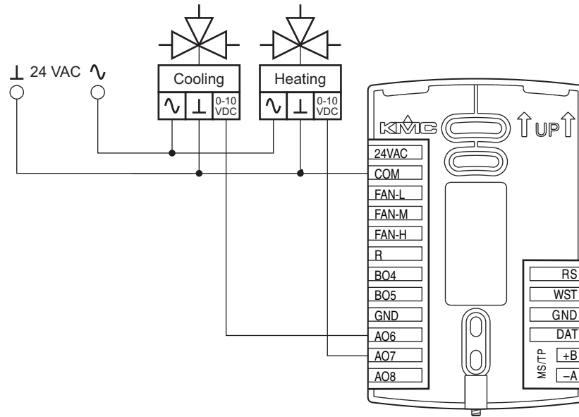
Illustration 2-11 Modulating heating and cooling valves
