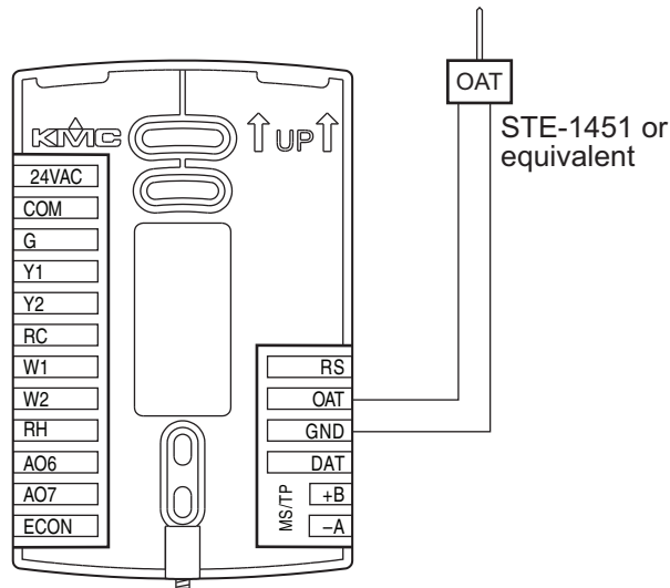
Illustration 2-7 Wiring for an outside air temperature sensor
