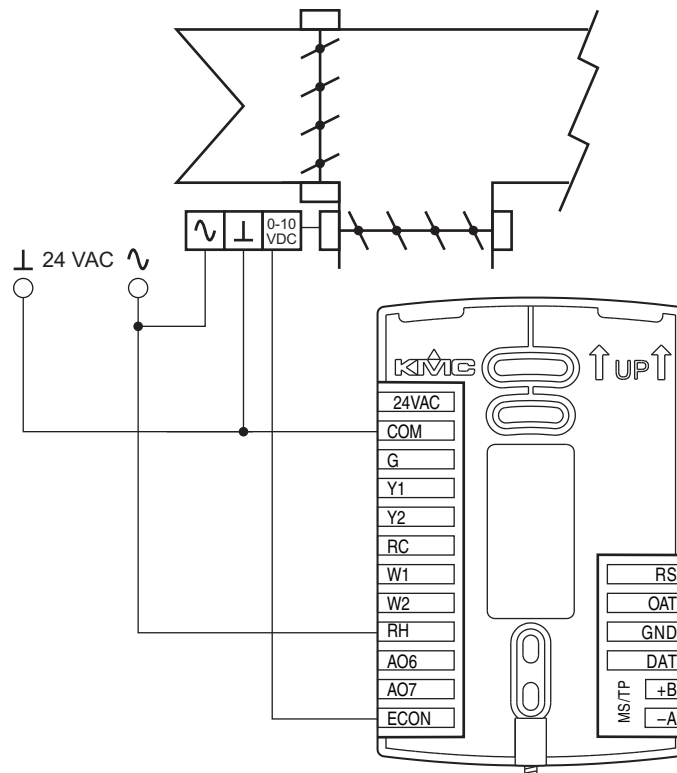
Illustration 2-12 Wiring for an economizer
